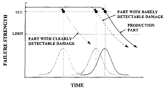
Figure 4 Impact of flaw tolerant flaws (50% probability)
