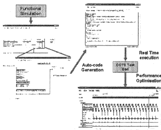
Fig. 10 Typical Rapid Prototyping Design Flow
