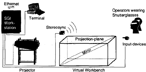
Fig. 5: Principle of a semi-immersive virtual workbench
