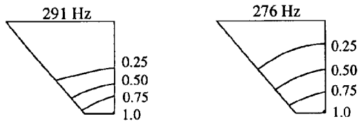
7a Fundamental bending
