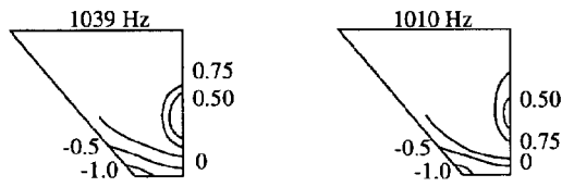
7c Overtone bending
