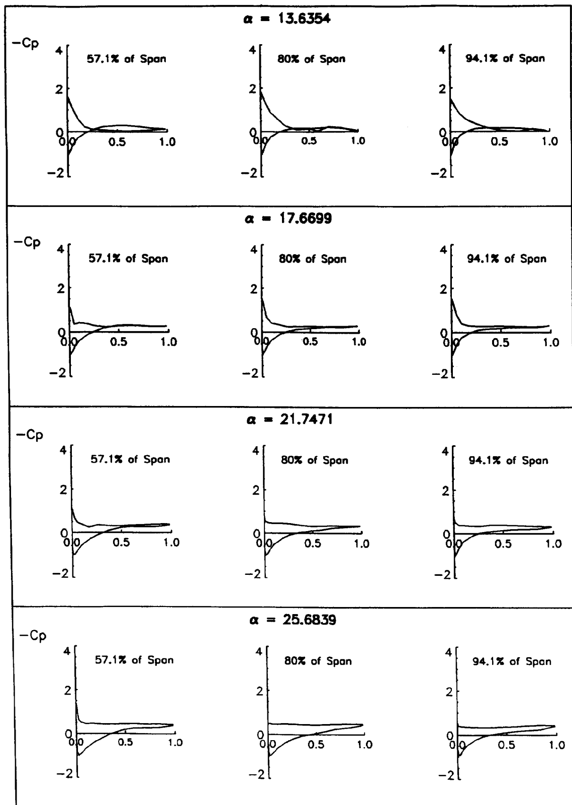
Fig 11 Chordwise pressure distributions (case 30681)
