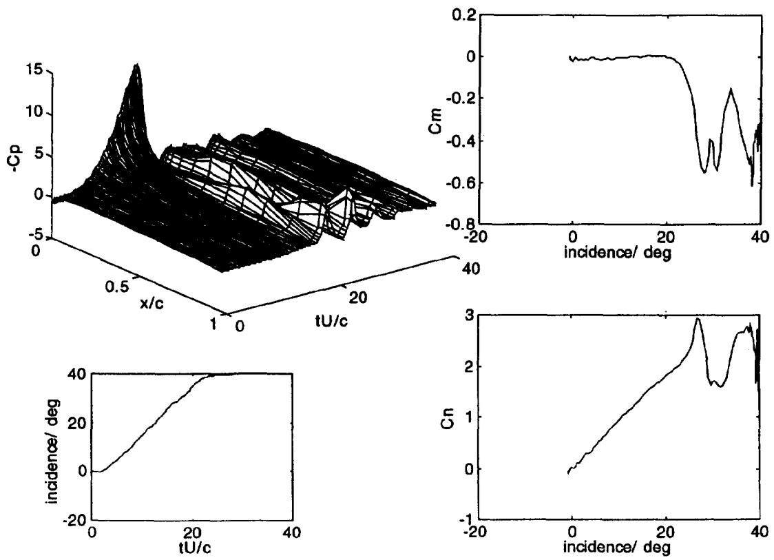
Fig 5 Pressure, normal force and pitching moment behaviour during ramp-up motion for the full chord NACA 0015. r=0.0187
