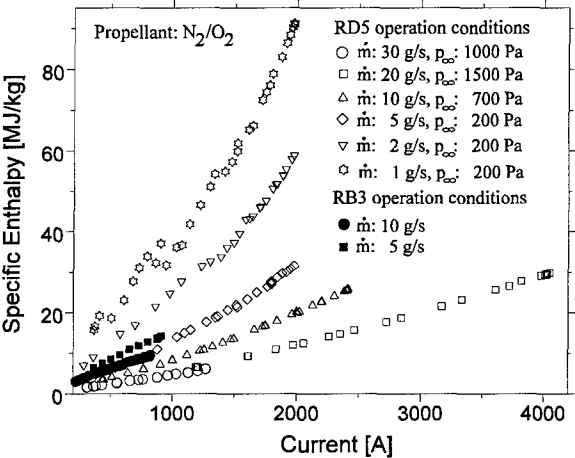
Fig. 4.13: Specific enthalpy vs. current for the MPG RD5 and the TPG RB3
