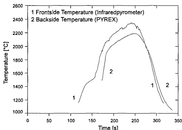
Fig. 2.5: Surface temperature of the ceramic heat shield of the EXPRESS capsule in the PWK
