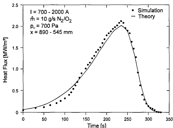
Fig. 2.4: Heat flux profile of the EXPRESS mission
