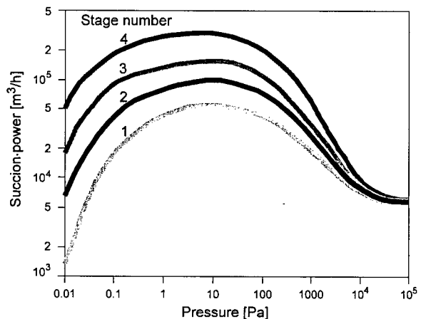
Fig. 3.11: Suction power of the vacuum system 1 m. The base pressure of the system is 0.5 Pa. The
