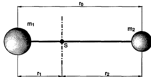
Fig. B2.9: Molecule as rotating dumb-bell
