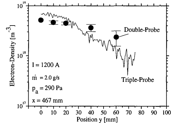
Fig. A7.14: Radial electron density distribution
