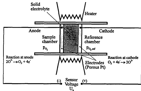
Fig. A6.2: Basic construction of a potentiometric solid state electrolyte sensor
