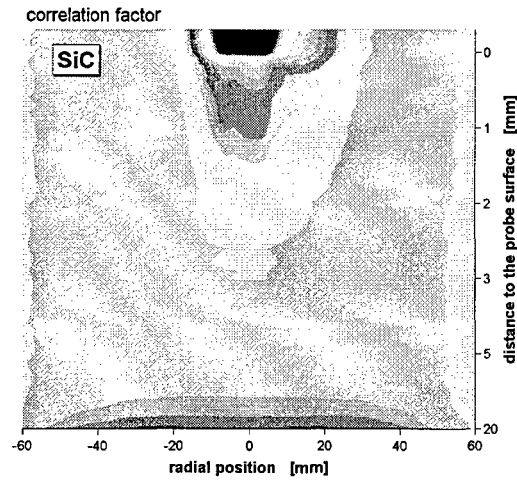
Fig. B2.18: Correlation factors in front of an SiC sample at 1280°C.
