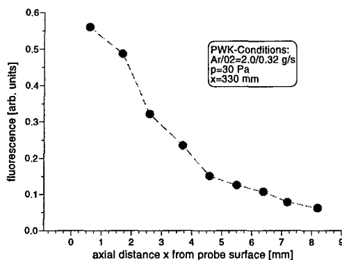
Fig. B5.15: Reaction zone of SiO in front of a silicon wafer
