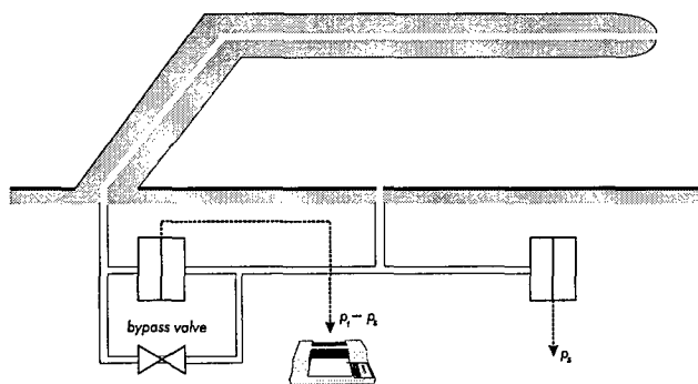
Figure 14. Pitot pressure measurement set-up (schematic drawing)
