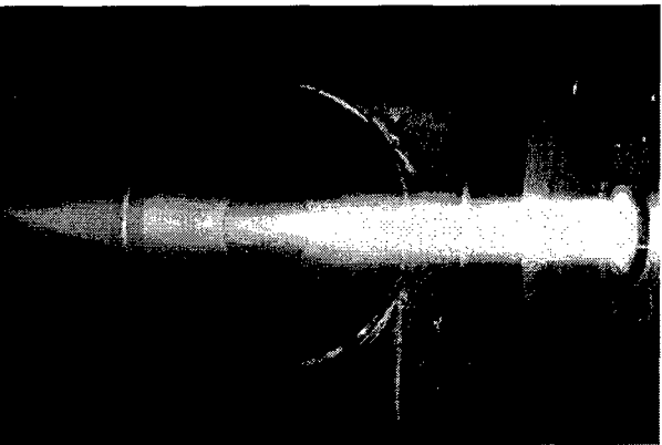
Figure 8. Air plasma jet from the 80 mm torch
