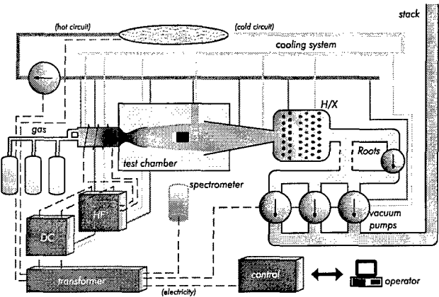
Figure 6. The Plasmatron facility (schematic drawing)
