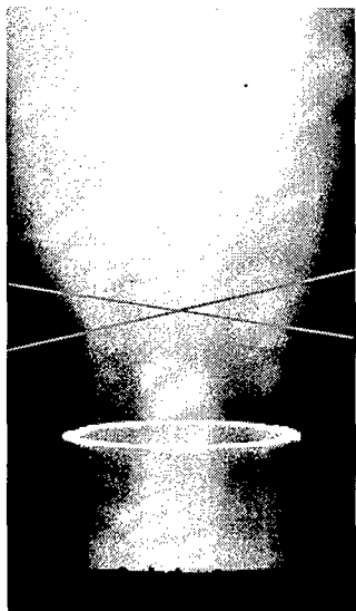
Figure 37. Crossing laser beams in the plasma jet
