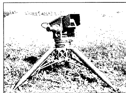
Figure 16 : Range Automatic Positioning Sensor
