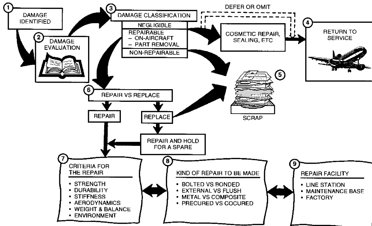
Figure 7. Damage Evaluation and Selection of Repair Methods
