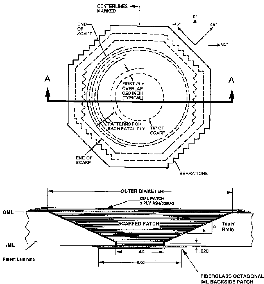
Figure 10. Scarfed Repair
