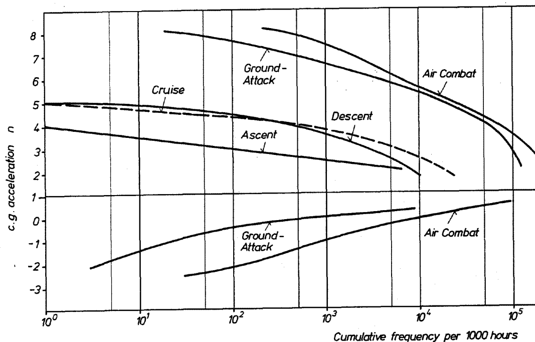
Fig. 2.1- 2 Typical Exceedance Curves for Combat Aircraft
