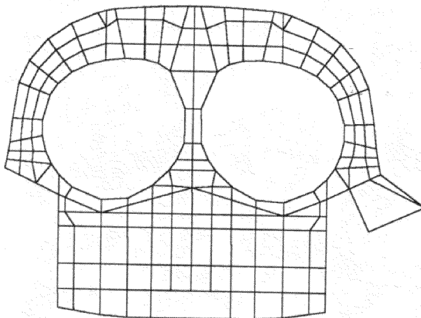
Fig. 2.2-4A Coarse Mesh FE-Model of Center Fuselage Frame
