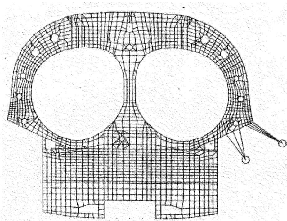
Fig. 2.2-4B Fine Mesh FE-Model for Detail Analysis
