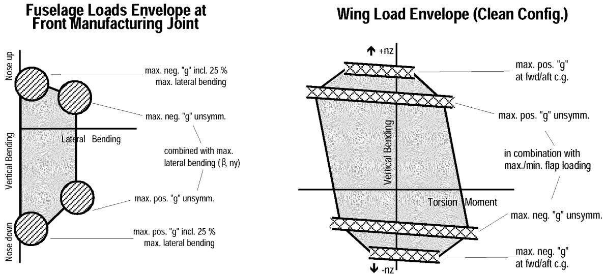
Fig. 1.2.5-2 Major Aircraft Component Loads Envelopes
