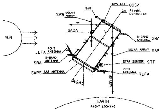
SAR Satellite in the orbit configuration
