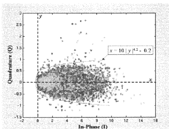
Fig. 9 Output signal from ATI processor, with clutter phases center around zero and moving target phases at non-zero values.
