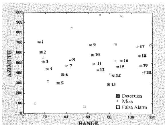
Fig. 8 Output of CFAR detector.
