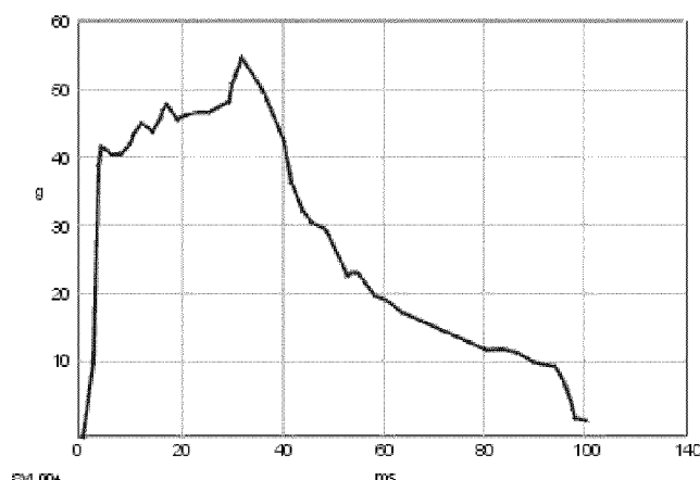
Figure 10 : Launch Accelerations
