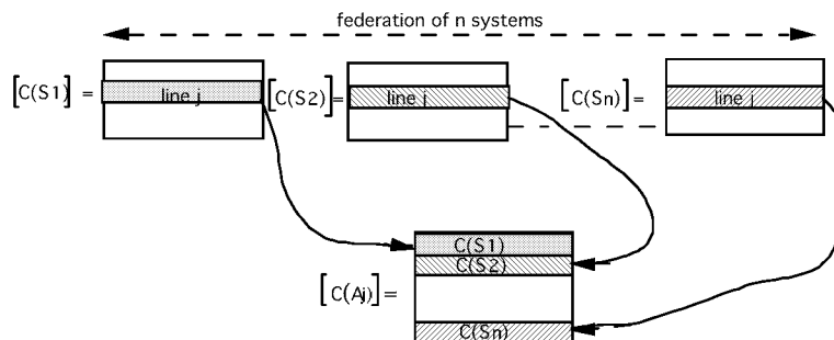
Fig. 9 Matrix of intercooperability-action
