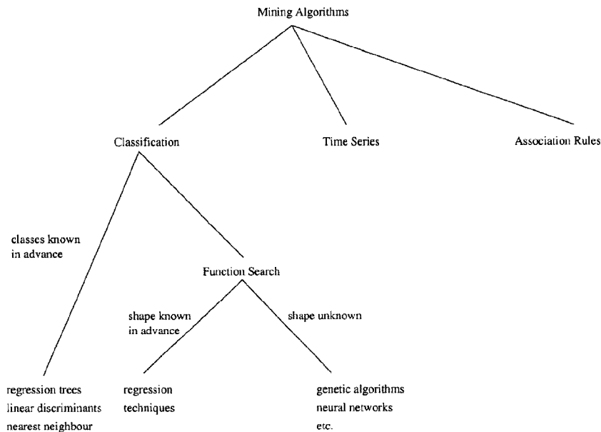
Figure 4: Module of mining algorithms
