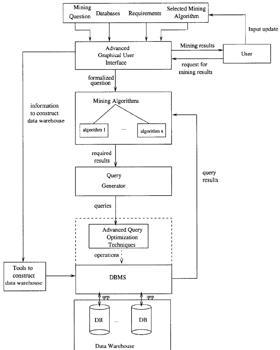
Figure 3: Architecture of a data mining tool
