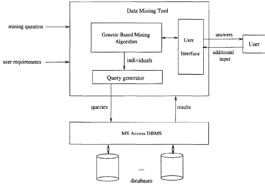
Figure 5: Architecture of SHARVIND
