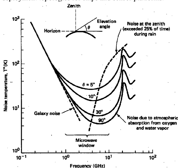
Figure 1 – Sky Noise temperature versus frequency (from [Skla-88])
