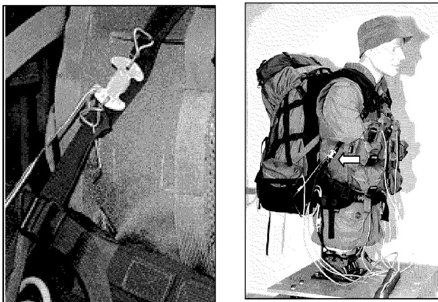
Figure 4. Custom strap force transducers for measuring strap tension.
