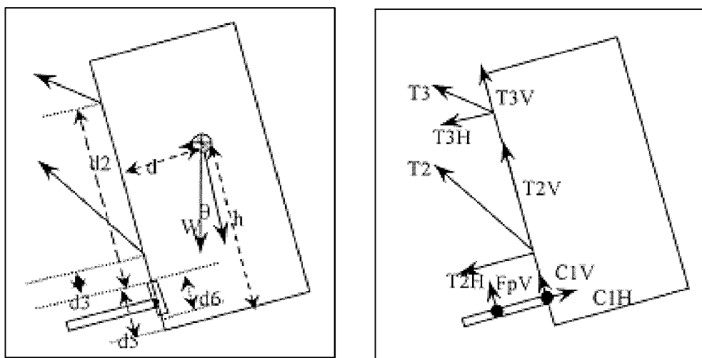
Figure 7. Static biomechanical pack model indicating input values (a-left) and outcome values (b-right)
