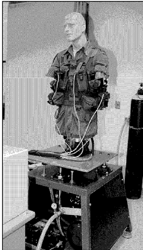
Figure 1. Dynamic Load Carriage Simulator (can be programmed to walk, jog or run and is set-up to test a load-bearing vest design)
