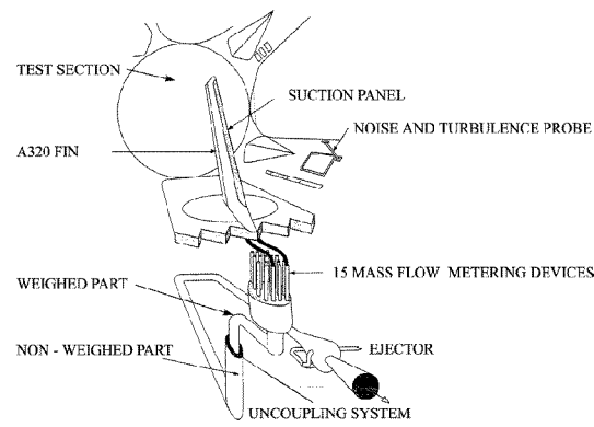
Fig. 6 – External suction device arrangement
