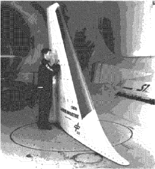
Fig. 5 – Test set-up of the A320 fin model
