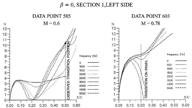
Fig. 11 – Stability analysis
