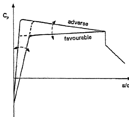
Fig 5 Sketch of Pressure Distributions
