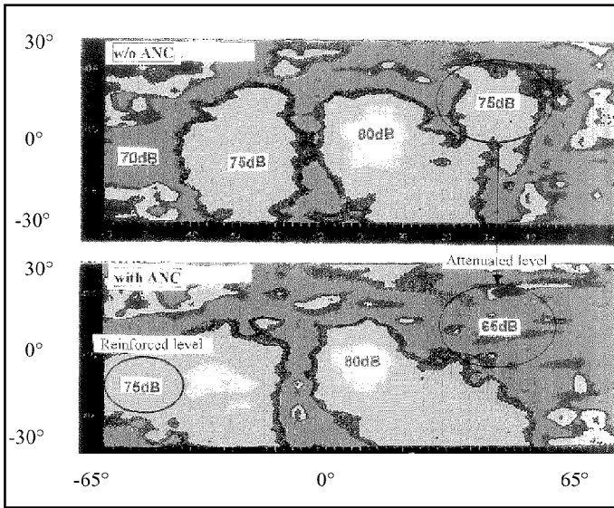
Fig 17 : Upstream far field map (1BPF/1700Hz)
