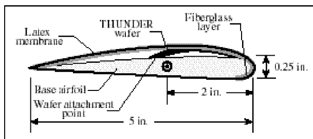
Figure 2. ATTACH testbed.
