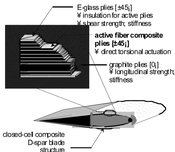
Figure 11: Full-scale active fiber composite rotor blade concept.
