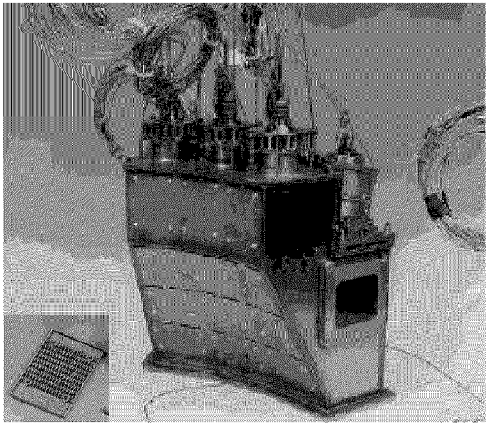
Figure 3 Test Combustor, cooling tile shown in inset
