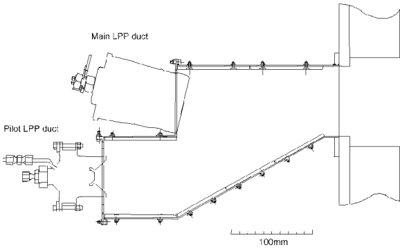
Figure 1 Axially Staged LPP Combustor
