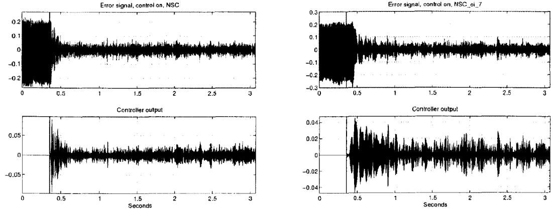
Figure 6: Error sensor (top) and control output (bottom) for a volume flow rate of 16 m³/h. On the left: reference algorithm, on the right: SAC scheme. Switch on of the control (vertical line).
