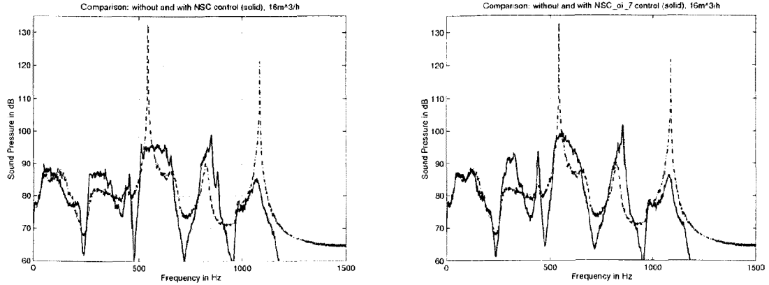
Figure 5: Pressure spectra (----) without and (—) with control. Volume flow rate of 16 m³/h. On the left: reference algorithm, on the right: SAC scheme.
