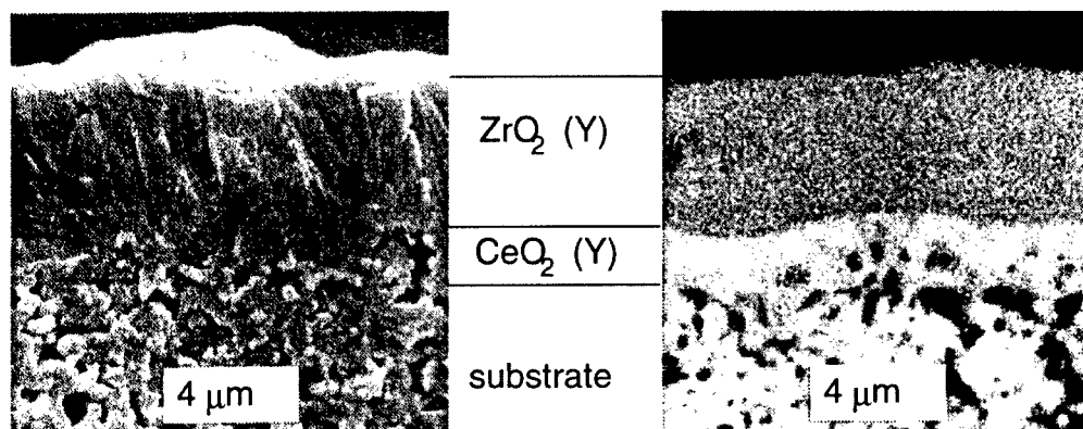
Fig. 8. SEM picture (left) and elemental analysis (right) of an electrolyte bilayer deposited via DC sputtering on top of a porous cathode substrate. It consists of a 1- \mu m thick CeO_2 (Y) chemical compatibility layer and a 4- \mu m thick ZrO_2 (Y) electrolyte layer [94].
