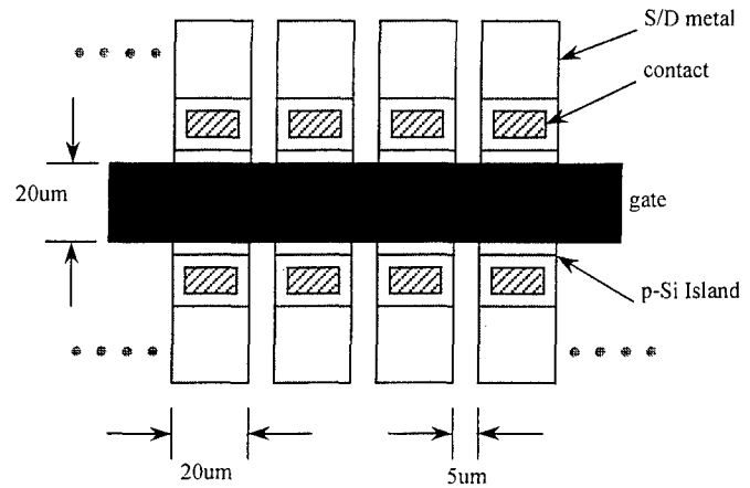
Figure 2. Design of continuous TFTs.
