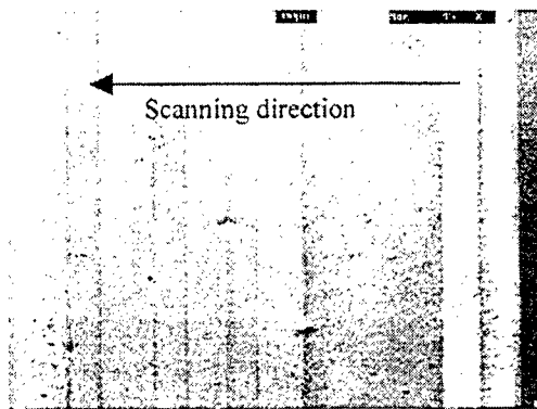
Figure 5 The SEM photograph of the laser crystallized poly-Si film with 75% laser overlapping ratio.
