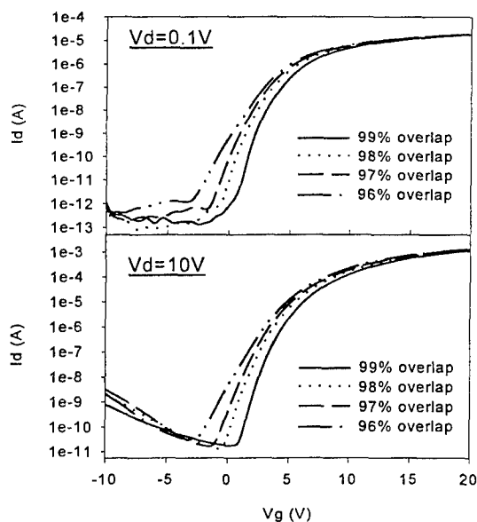
Figure 9 The typical I_d - V_g curves ( V_d=0.1 and 10 volt) of n-type single-gate TFT ( W/L = 50/20\mu m ) with various laser overlapping ratios (96%~99%).
