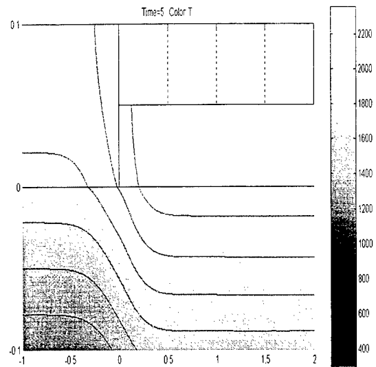
Fig. 2 Simulation of a temperature profile, in Kevine degree, at the edge of a recessed silicon film after laser irradiation. The upper region above zero is silicon and the bottom, silicon dioxide.
