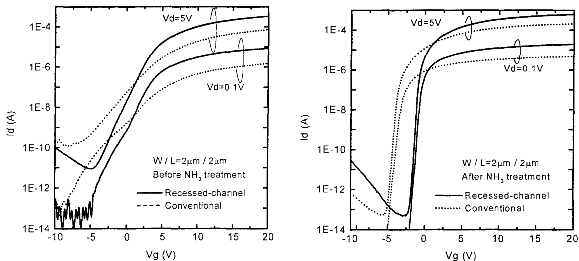
Fig. 4 I_d - V_g curves of 2- \mu\text{m} recessed and conventional TFTs before (left) and after (right) \text{NH}_3 plasma treatment.
