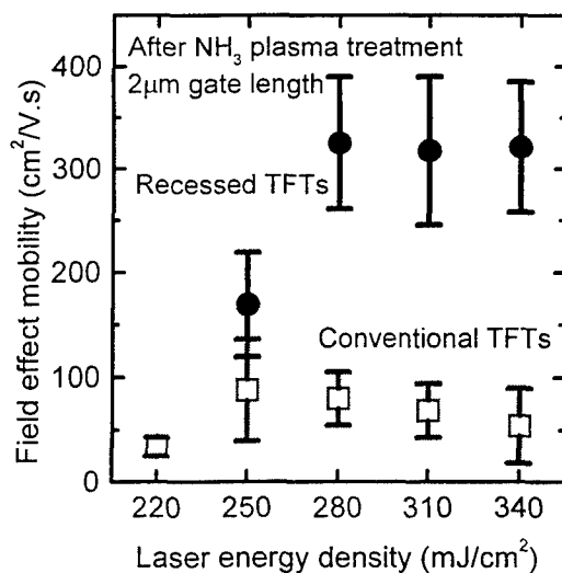
Fig. 6 The comparison of field-effect mobilities of recessed and conventional TFTs prepared with different laser energy densities.
