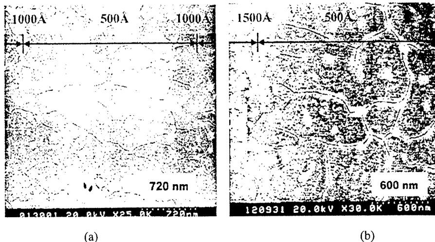
Fig. 3 The SEM micrographs of Secco etched ELC recessed-structure silicon films.
