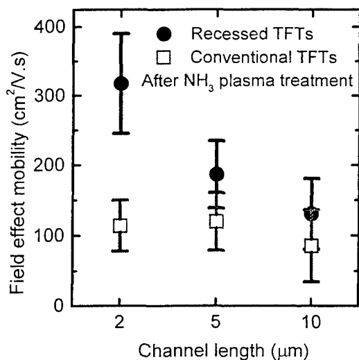
Fig. 5 The comparison of field-effect mobilities of recessed and conventional TFTs with different channel lengths.
