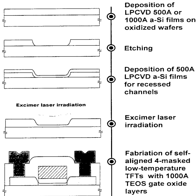
Fig. 1 The brief process flow of recessed TFTs.
