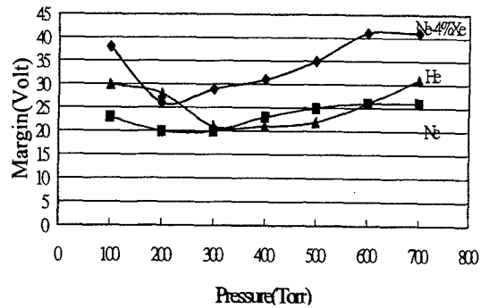
Fig. 9 The memory margins with pressures in different gas.
