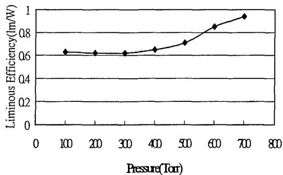
Fig. 5 The luminous efficiency with Ne-4%Xe gas pressure.
