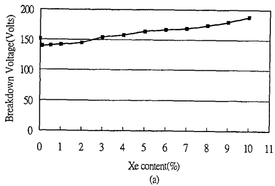
Fig. 7(a) The breakdown voltage with Xenon percentage.
