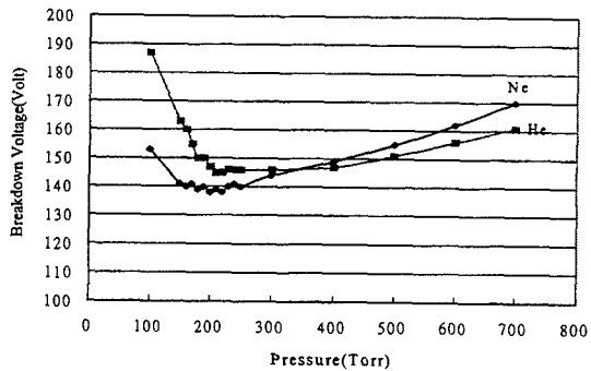
Fig. 8 The breakdown voltages for Helium and Neon at different gas pressure.
