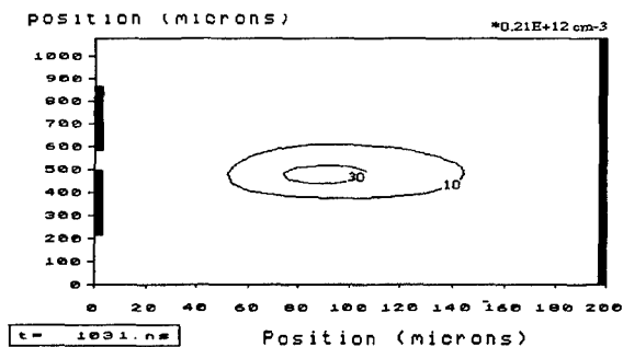
Fig. 10(a)-(d) Two-dimensional simulation of Ne4%Xe and Ne-10%Xe gas. Profiles of (a) electron density, (b) ion density, (c) excitation rate, (d) electric potential.
