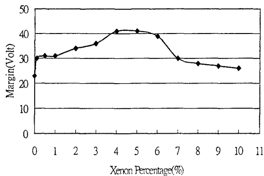
Fig. 1 The memory margin with Xenon percentage in Ne-Xe gas at 500Torr..
