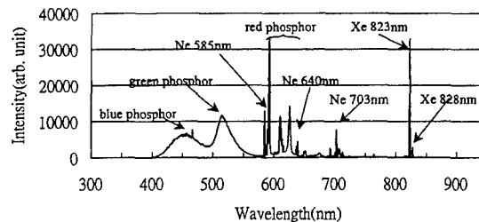
Fig. 4 The spectra emission from PDP cells with Ne-4%Xe gas at 500Torr.
