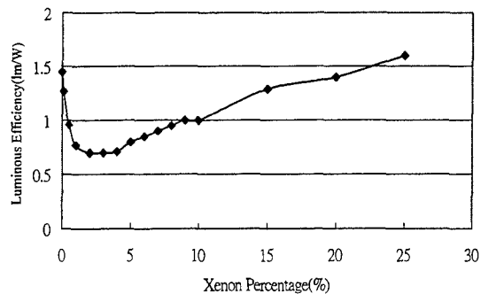
Fig. 2 The luminous efficiency with Xenon content in Ne-Xe gas at 500Torr.
