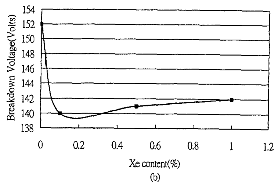
Fig. 7(b) The breakdown voltage with Xenon percentage.
