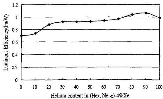
Fig. 6 The luminous efficiency in (Hex, Ne1-x)-4%Xe gas at 500Torr.
