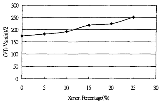
Fig. 3 The operation voltage with different Xenon content in Ne-Xe gas at 500Torr.
