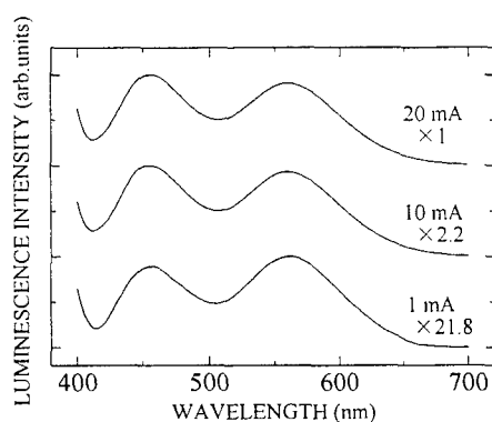
Fig.3 Emission spectra of \text{ZnS}:\text{Cu},\text{Al} phosphor obtained at RT at three different forward-bias currents (1, 10 and 20 mA)
