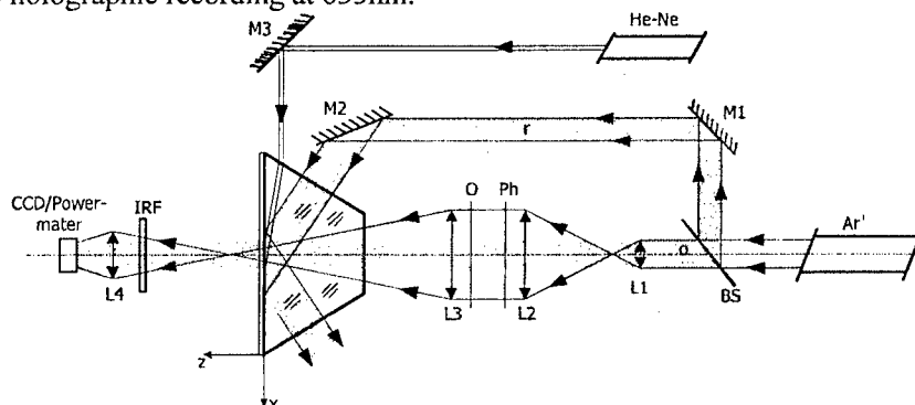
Fig. 2. Optical arrangement for evanescent-wave holographic recording: L-lenses; M-mirrors; BS-beam splitter; Ph-phase mask; O-object; IRF-interference red filter.
