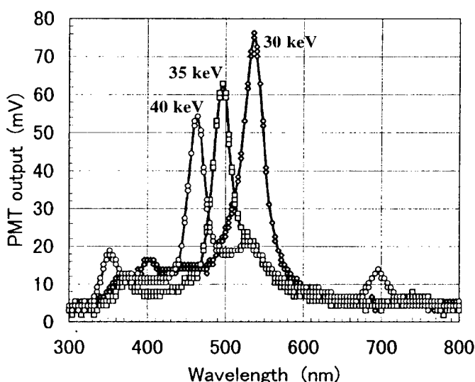
Fig. 5: Power spectra of Smith-Purcell radiations for several beam energy
