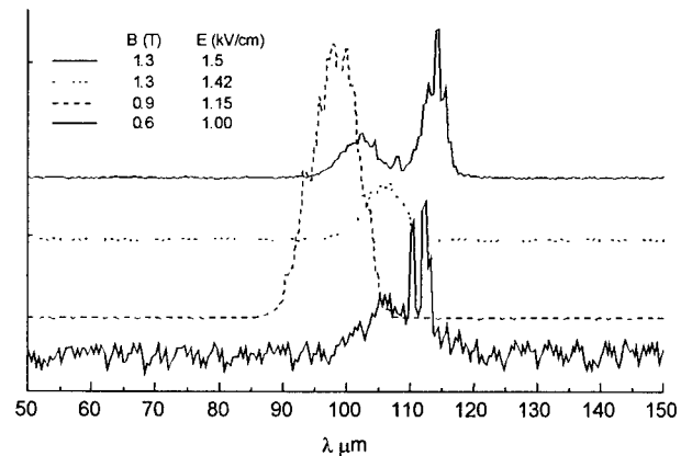
Fig. 6: Emission spectra at various B fields.
