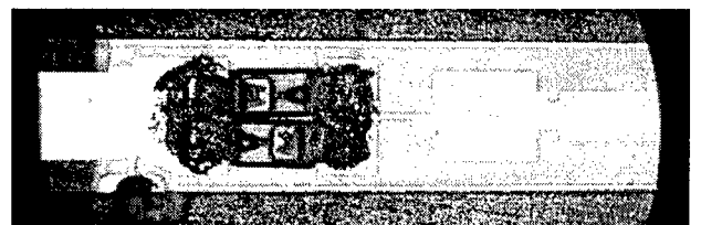
Fig. 2: Beam Lead diodes bonded on a 0.420 mm width quartz substrate of 80µm thickness.
