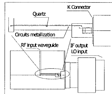
Fig. 1: Structure of the harmonic mixer bloc.
