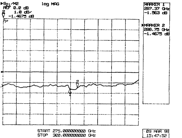
Fig.10: Low loss measurement of the transmission through a WR3 H-Bend and a WR3 coupler. Scale: 1 dB / Div between 275 to 300 GHz.
