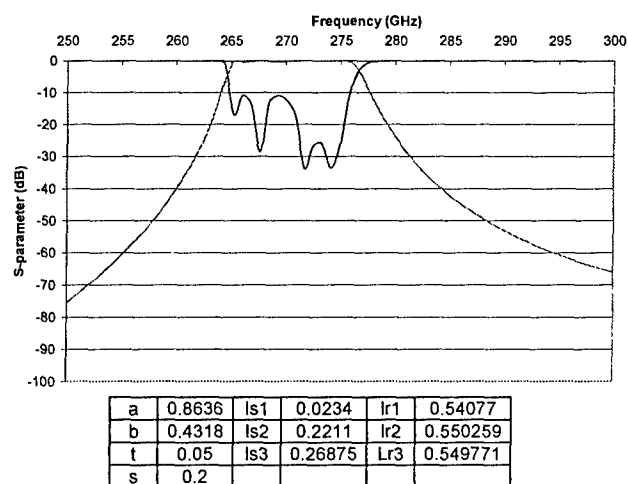
Fig. 3: Dimensions and performance of 270GHz bandpass filter
