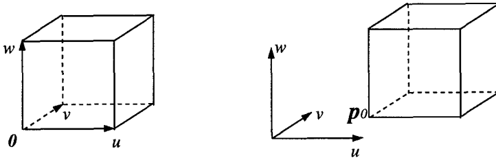
Fig. 2. Translating the coordinate system of a voxel.
