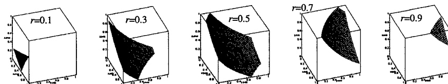
Fig. 4. Contours of a voxel with S(V) = 1 .
