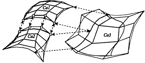
(b) The control polyhedrons of Ca1 and Ca2 can be merged to form one bar network because they are connected along their entire boundary whereas Ca3 generates another bar network since Ca3 is connected to Ca1 and Ca2 along a trimming line.
