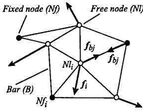
(a) An example of bar network
