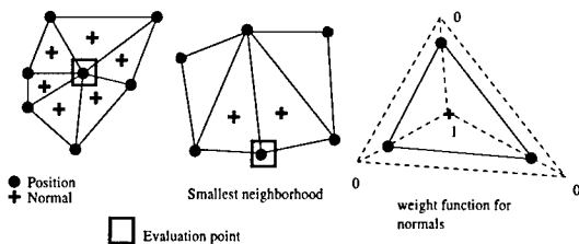
Fig. 1. Neighborhood selection.
