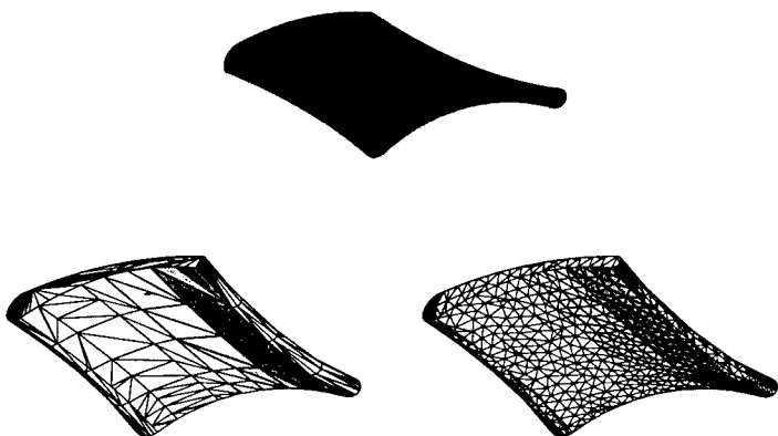
Fig. 5. Edge flipping and node insertion.
