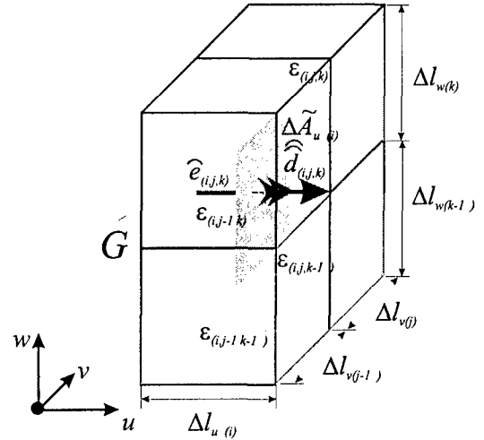
Fig. 3. Relation of electric flux \hat{d} with electric voltage \hat{e} in conventional FIT .
