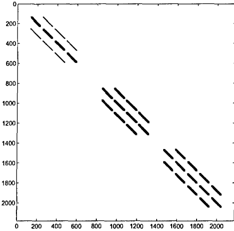
Fig. 8. Structure of the 15-banded M_{\epsilon}^{-1} matrix of a cavity discretized with 10 \times 10 \times 5 cells and PEC boundary.
