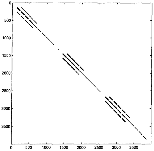
Fig. 15. Structure of a mixed second-fourth order M_{\varepsilon-1} matrix of a cavity discretized with 10 \times 10 \times 10 cells and PEC boundary. Half of the calculation domain is discretized with the fourth order approach, the other one with conventional second order scheme.
