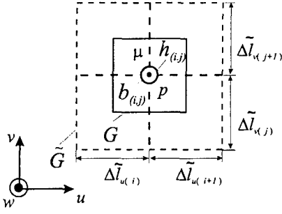
Fig. 5. Local transformation of tangential continuous magnetic field strength into normal continuous magnetic flux density at the intersection point p of normal facet and dual edge.
