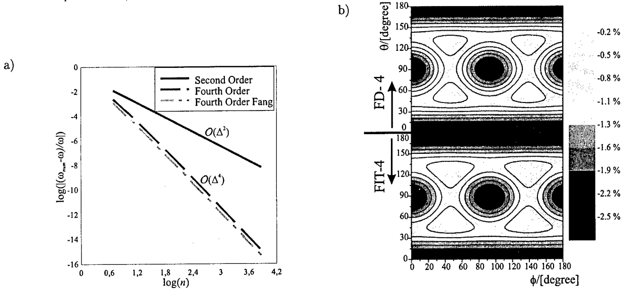
Fig. 12. Convergence of the spatial dispersion relation (27) to the exact solution in (28). Figure a) displays the relative error of the angular frequency \omega_{num} of a plane wave traveling diagonally through the grid using second and fourth order material matrices and also the FD-4 operator in dependence of the number of grid steps per wavelength ( n = \lambda/\Delta ). Fig. b) displays the relative phase error in percent of the FIT-4 scheme (lower part) and of the FD-4 scheme (upper part) at a sampling rate of n = \lambda/\Delta = 4 as a function of the direction of wave propagation in the grid.
