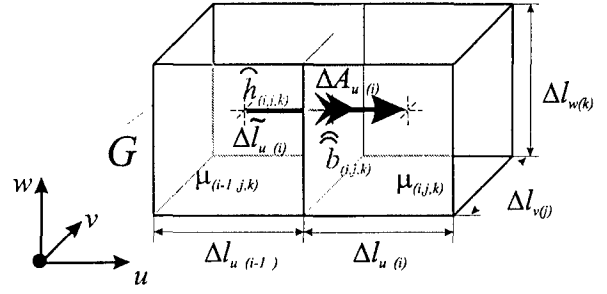
Fig. 2. Relation of magnetic flux \hat{b} with magnetic voltage \hat{h} in conventional FIT .
