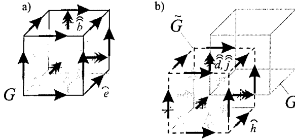
Fig. 1. Location of electric voltage \bar{e} on edges and magnetic flux \bar{b} on facets of primary grid G (a) and magnetic voltage \bar{h} on edges and electric flux \bar{d} and electric current \bar{j} on facets of dual grid \tilde{G} (b).
