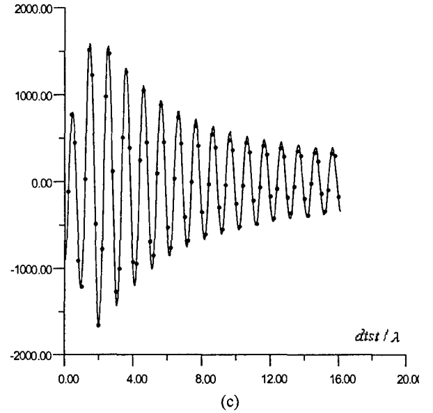
Figure 3. The backscattered electric field with distance ( dist is the distance from the surface of the cube) for normal plane wave incidence on a cube (side length L_x = L_y = L_z = 2.4\lambda ), \vec{E}^{inc} = 1000 \sin 2\pi f_0 t \hat{x} , f_0 = 900 \text{ MHz} , — Yee results ( R=20 ).
