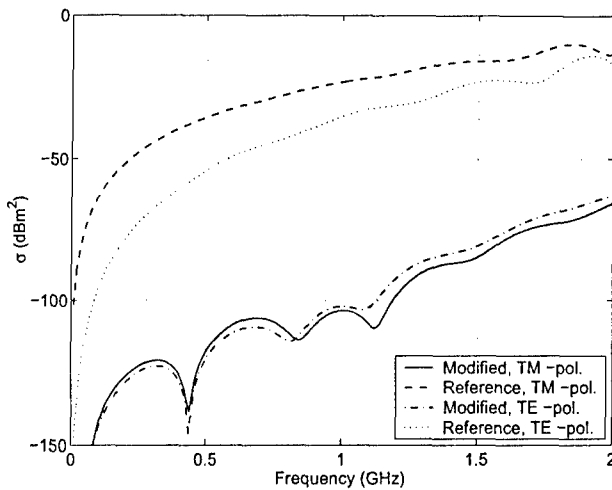
Figure 8: Bistatic RCS of empty FDTD volume as function of frequency. Incidence angle \theta_i = 45^\circ , \phi = 0^\circ . Scattering in specular direction. Both TE- and TM- results are shown.
