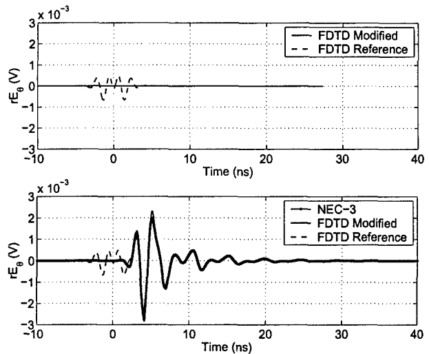
Figure 12: Time response of the monostatic scattering from a buried dipole 0.205 m below the ground level (bottom) and without dipole (top). Incidence angle \theta_i = 45^\circ , \phi = 0^\circ . TM-polarization.
