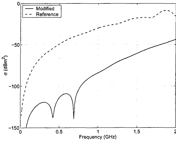
Figure 6: Monostatic RCS of empty FDTD volume as function of frequency. Incidence angle \theta_i = 0^\circ .
