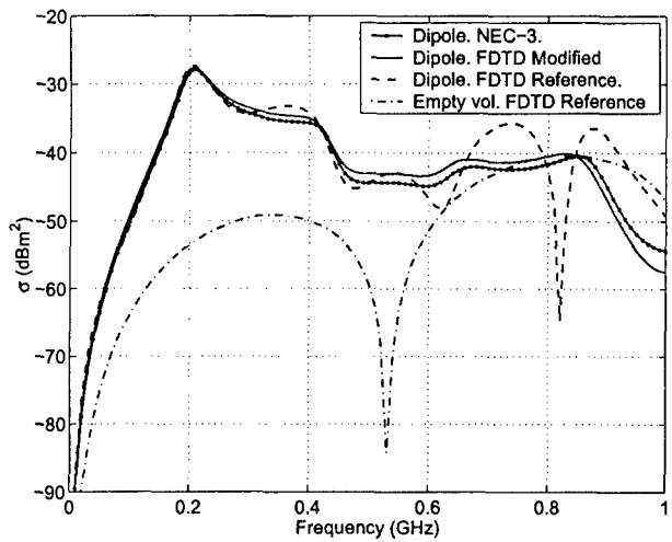
Figure 11: Monostatic RCS of buried dipole 0.205 m below the ground level. Incidence angle \theta_i = 45^\circ , \phi = 0^\circ . TM-polarization.
