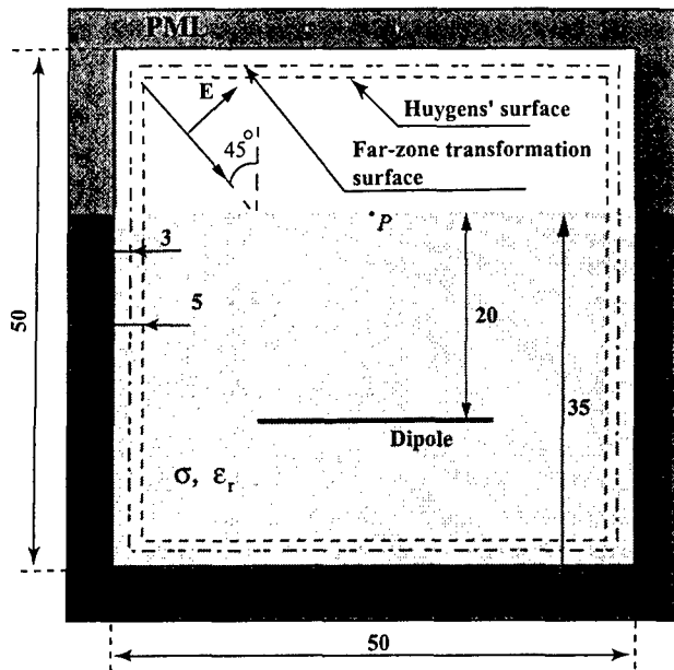
Figure 10: X-Z slice of the computational volume at y = 20\Delta y for the dipole case. The Huygens' surface extends 30 cells below the ground. The far-zone transformation is performed in the scattered field region 2 cells outside the Huygens' surface. The dipole is positioned 20 cells below the ground level (of tangential electric field components in FDTD)
