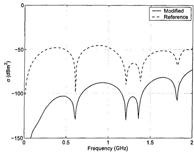
Figure 9: Monostatic RCS of empty FDTD volume as function of frequency. Incidence angle \theta_i = 45^\circ , \phi = 30^\circ . TM-polarization.
