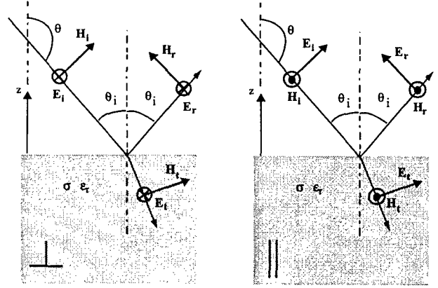
Figure 1: Reflection and refraction at an interface between free space and a homogeneous half space. Left: Polarization perpendicular to the plane of incidence. Right: Polarization parallel to the plane of incidence.
