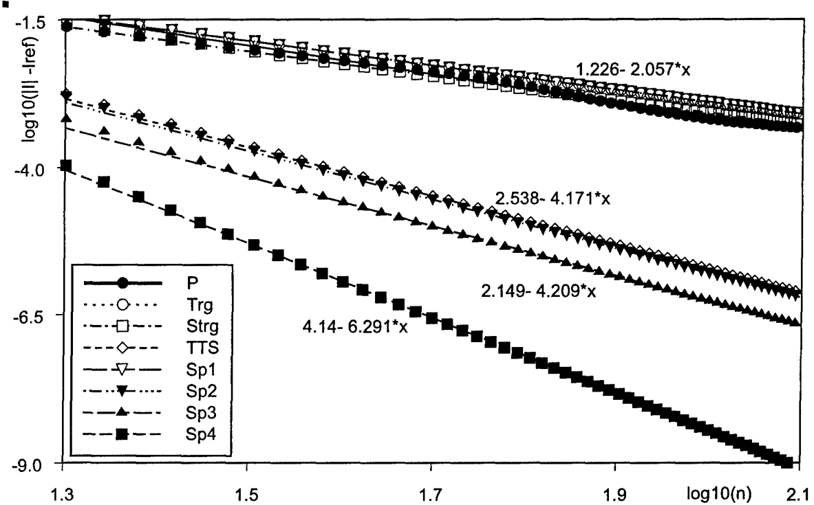
Figure 1b. Plots of \log_{10}(\|I\| - I_{ref}) versus \log_{10}(n) for eight expansion functions, using uniform cell sizes on an infinite cylinder. The regression values are associated with the four splines.
