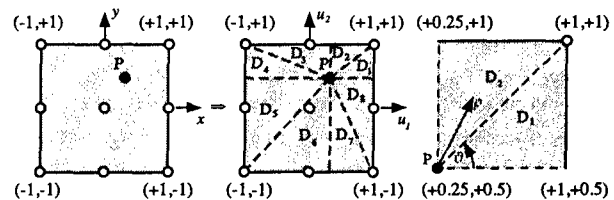
Figure 10 Surface element ( z = 0 ) and representation with normalized, local coordinates. The rectangle is subdivided into four quadrangles composed of two triangles each.
