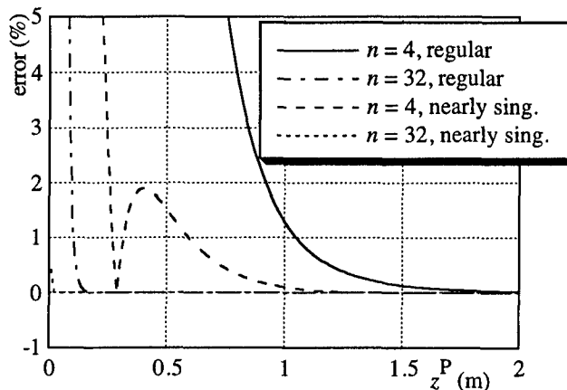
Figure 14 Nearly singular integrand. Error curves for the methods in 4.1 and 4.4 and an increasing number of nodes with observation point at various distances to the surface element.
