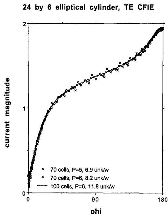
Figure 7. Results from the LCN method using a 70-cell model of an elliptical cylinder of dimensions 24\lambda by 6\lambda .
