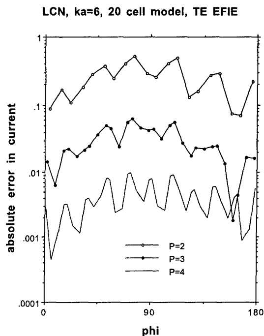
Figure 2. The error in the LCN current for a circular cylinder, ka=6 . A 20-parabolic-cell model is used with 2, 3, and 4 points per cell.
