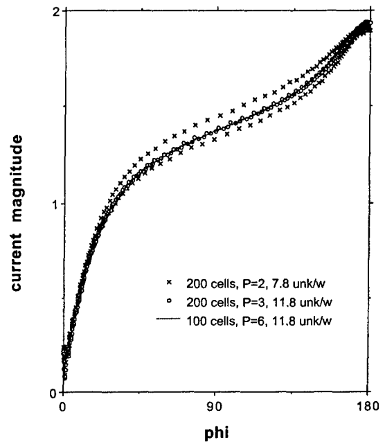
Figure 5. Results from the LCN method using a 200-cell model of an elliptical cylinder of dimensions 24\lambda by 6\lambda .
