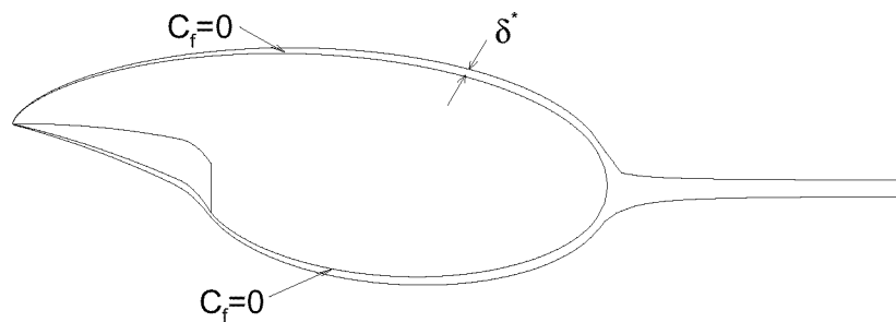
Figure 12: Super-cavitating hydrofoil with its boundary displacement thickness.
