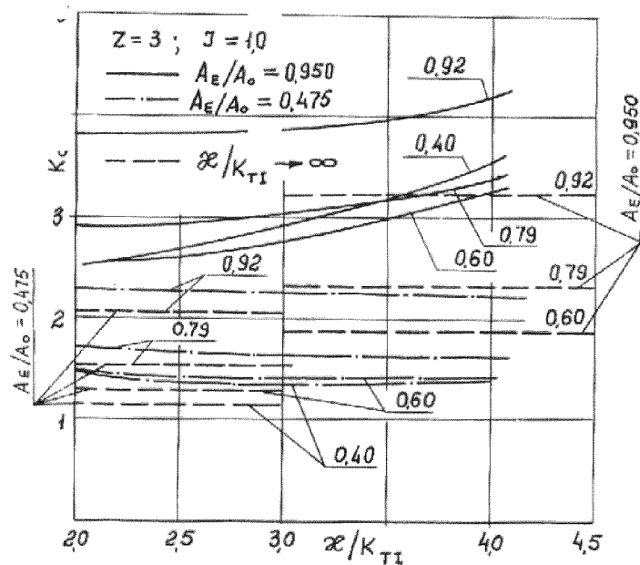
Fig.19. Correction for the camber of the blade cylindrical section central line together with the cavity (comparative data of supercavitating and non-cavitating propellers) [50]
