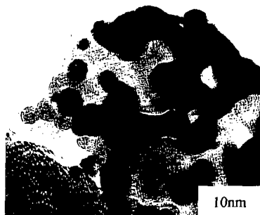
Fig.2 Onion-like fullerenes induced under 10% Pt nanoparticles by an electron irradiation at an intensity of 3.3 \times 10^{20} \text{ e/cm}^2 \text{ sec} for 2800 sec
