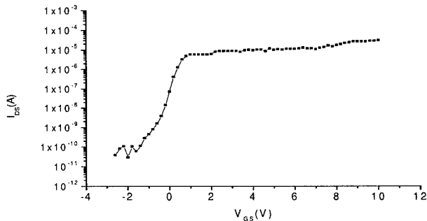
Fig. 6 TGF data for a transistor made from nc-Si
