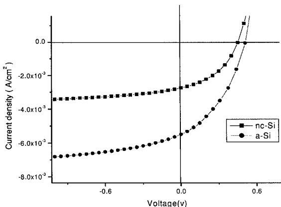
Fig. 7 nc-Si and a-Si solar cell J-V curve under 50 mW/cm 2 light.
