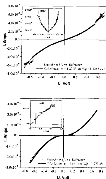
Figure 4. IV curves of Ni/NiO/Co nanowires of 30 nm diameters. Inserts are derivatives of the curves, with the corresponding fittings using tunneling (left) of Coulomb blockade at low bias and tunneling at high bias (right).
